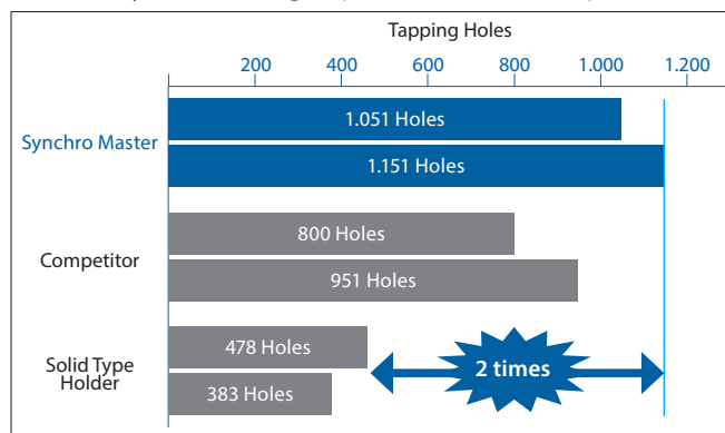
Work Material: SCM440 (30HRC) Tool: S-XPf M10x1.5 2P Cutting Speed: 15m/min
